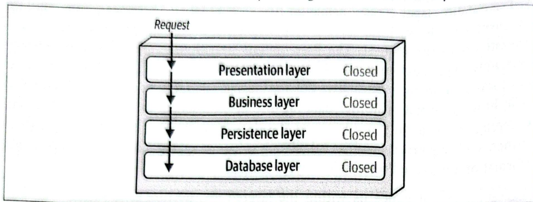
Figure 10-3. Closed layers within a layered architecture
